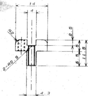
B-B CROSS SECTION
